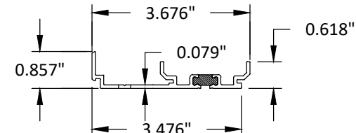
72 STRAP ANCHOR 6063-T5 MINIMUM 4 1/2" LENGTH
