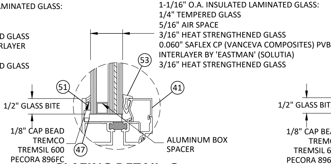
GLAZING DETAIL G
