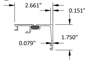
8 RECEPTOR 6063-T5
