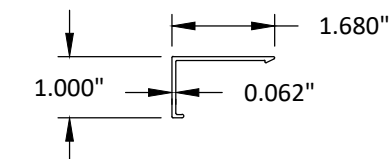
69 1" X 1 11/16" COVER 6063-T5
