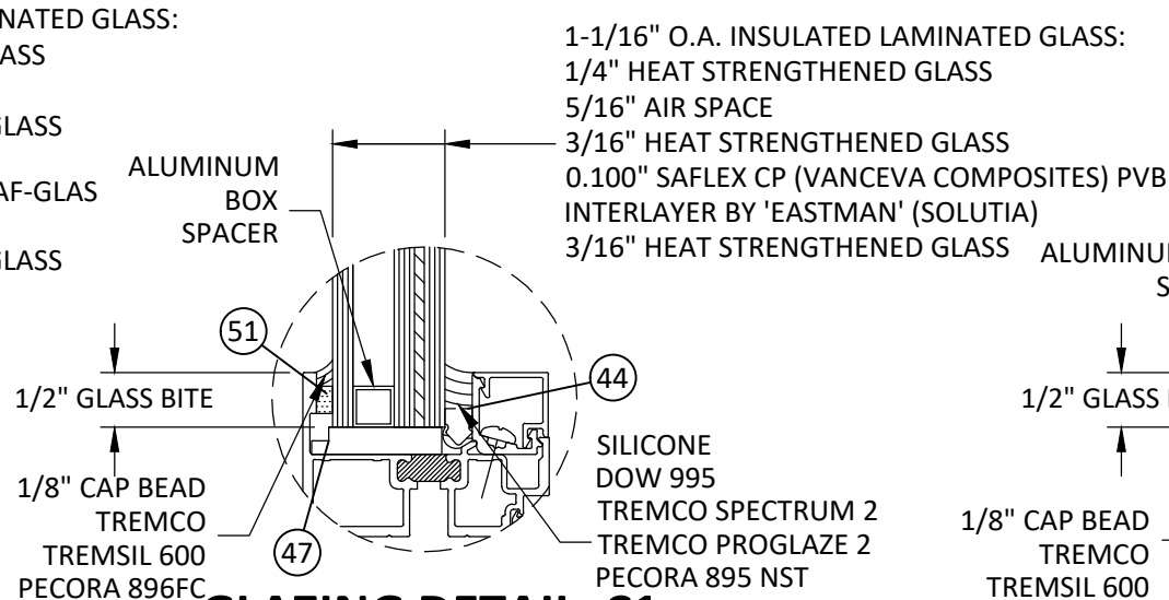
GLAZING DETAIL C1
