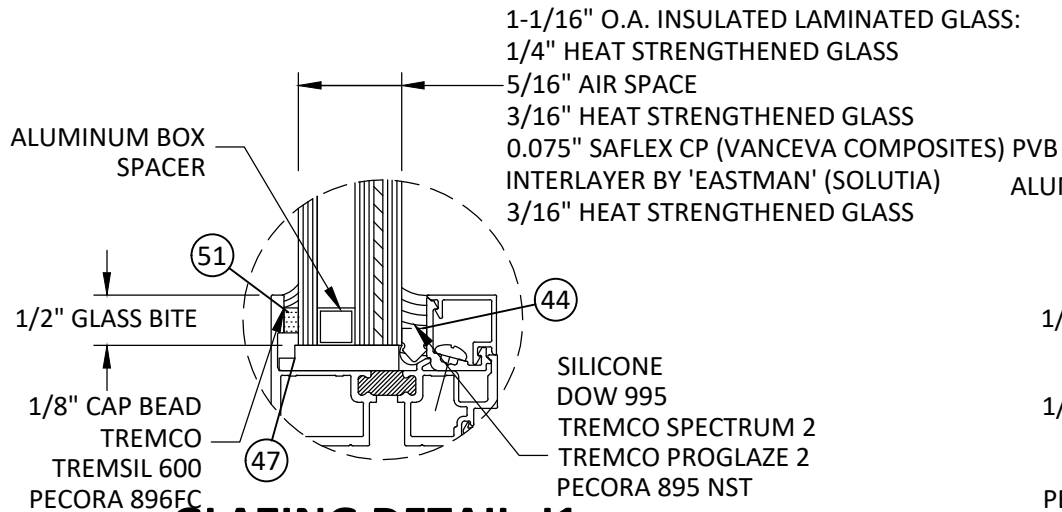
GLAZING DETAIL I1
