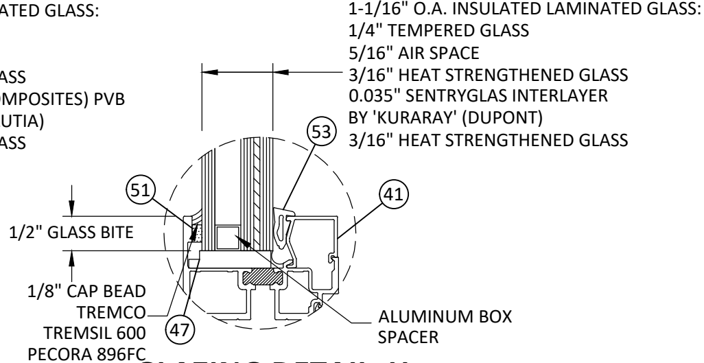
GLAZING DETAIL H
