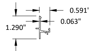
11 FIXED GLASS STOP 6063-T5
