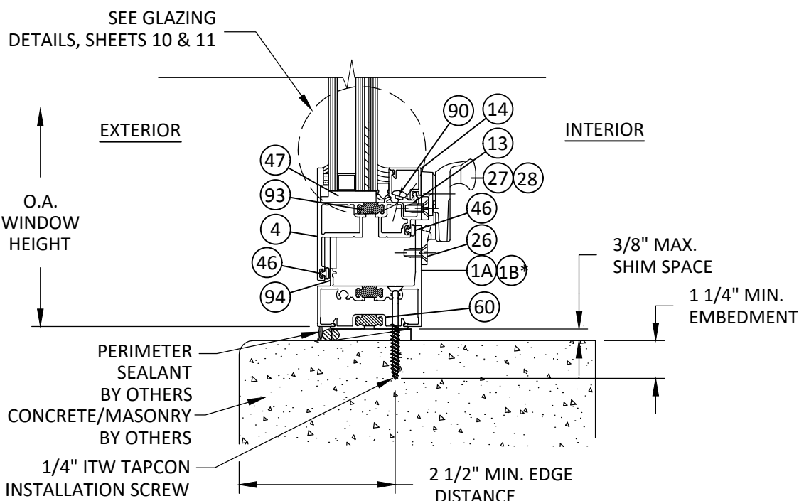
N 7 VERTICAL SECTION VENT SILL - CONCRETE/MASONRY THROUGH FRAME - TYP.
