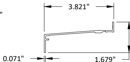
15 3" SILL TRIM 6063-T5
