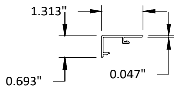
12 FIXED SNAP COVER 6063-T5
