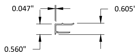
22 FIXED GLASS STOP COVER 6063-T5
