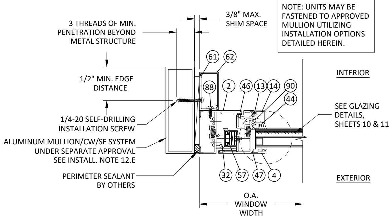
T 8 HORIZONTAL SECTION VENT JAMB - MULL TUBE FRAME TRIM CLIP ANCHOR - TYP.
