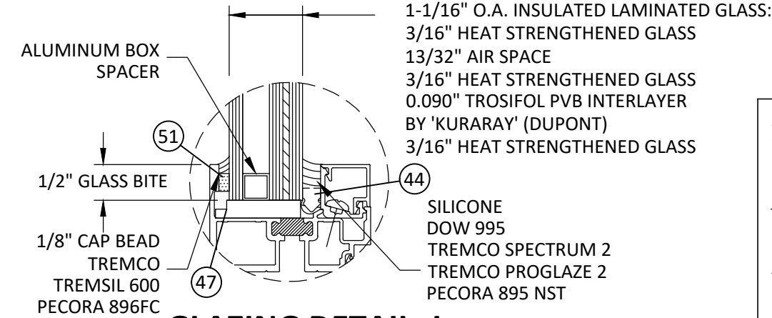
GLAZING DETAIL J
