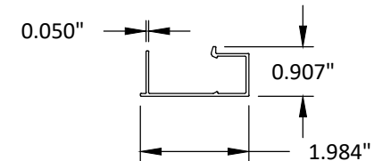
67 STRAP ANCHOR COVER 6063-T5
