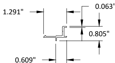
21 FIXED GLASS STOP 6063-T5
