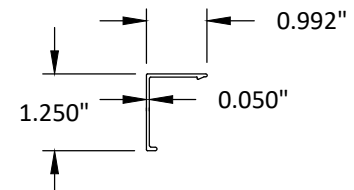
66 1 1/4" X 1" COVER 6063-T5
