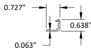
13 VENT GLASS STOP 6063-T5
