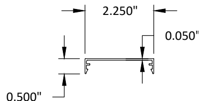
20 COVER 6063-T5
