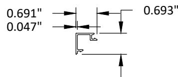
14 VENT SNAP COVER 6063-T5
