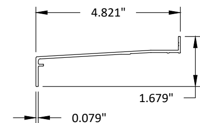
102 4" SILL TRIM 6063-T5
