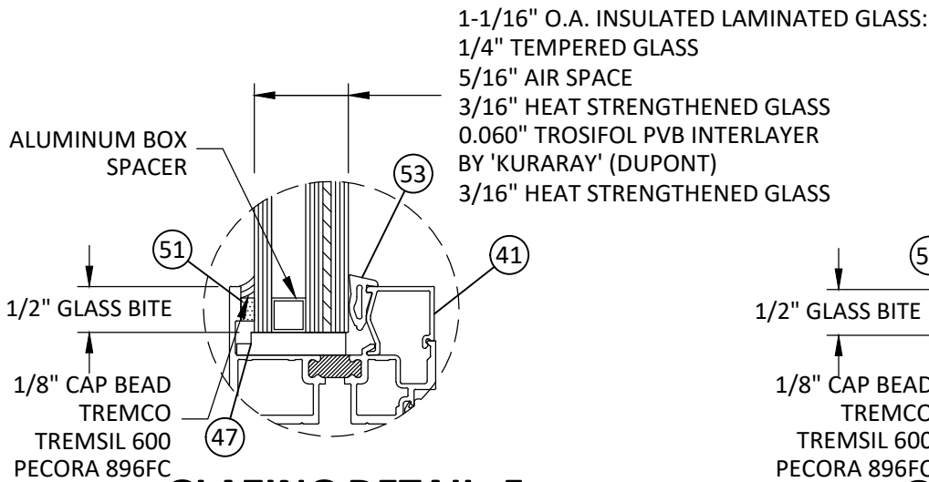
GLAZING DETAIL F
