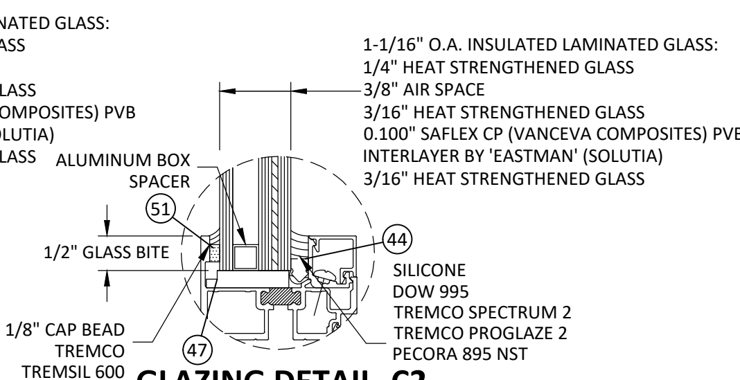
GLAZING DETAIL C2
