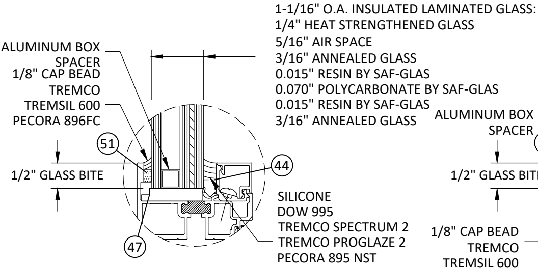
GLAZING DETAIL A1
