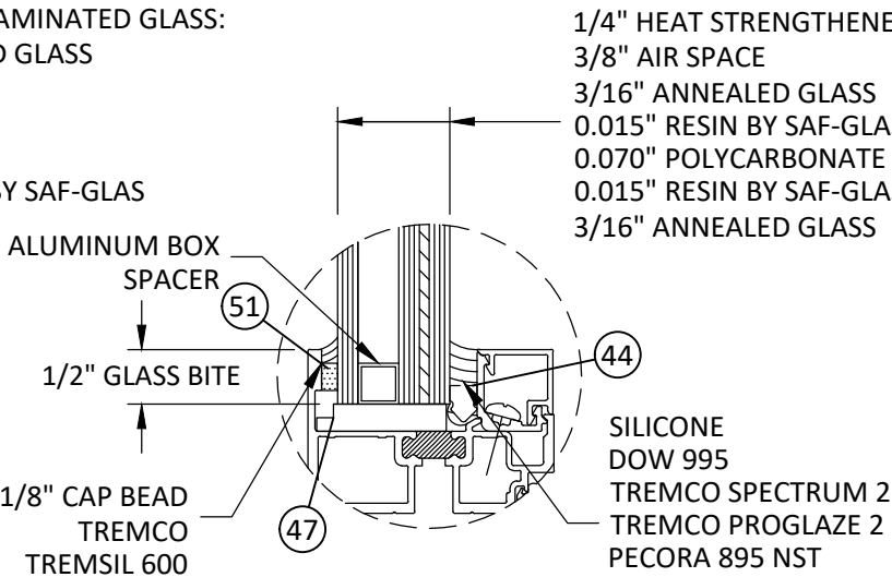
GLAZING DETAIL A2
