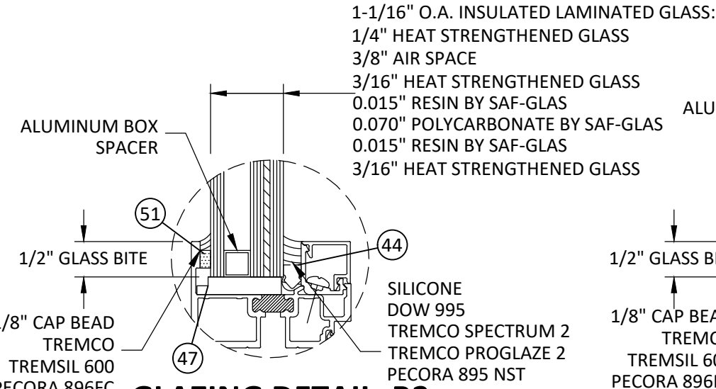
GLAZING DETAIL B2
