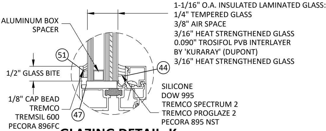
GLAZING DETAIL K
